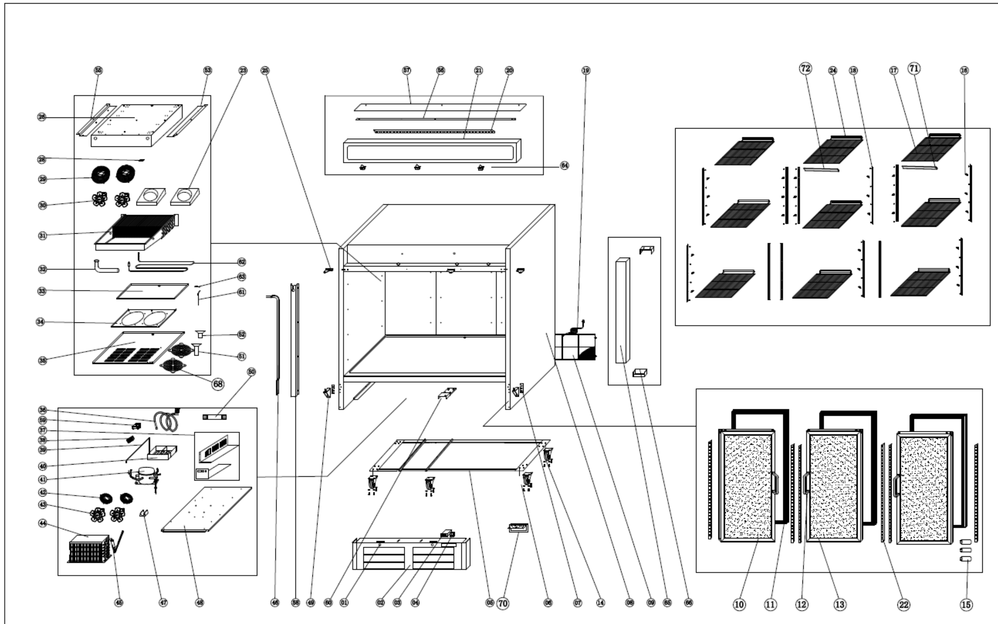
EXPLODE OF KCHGM72F (R404a Version)
